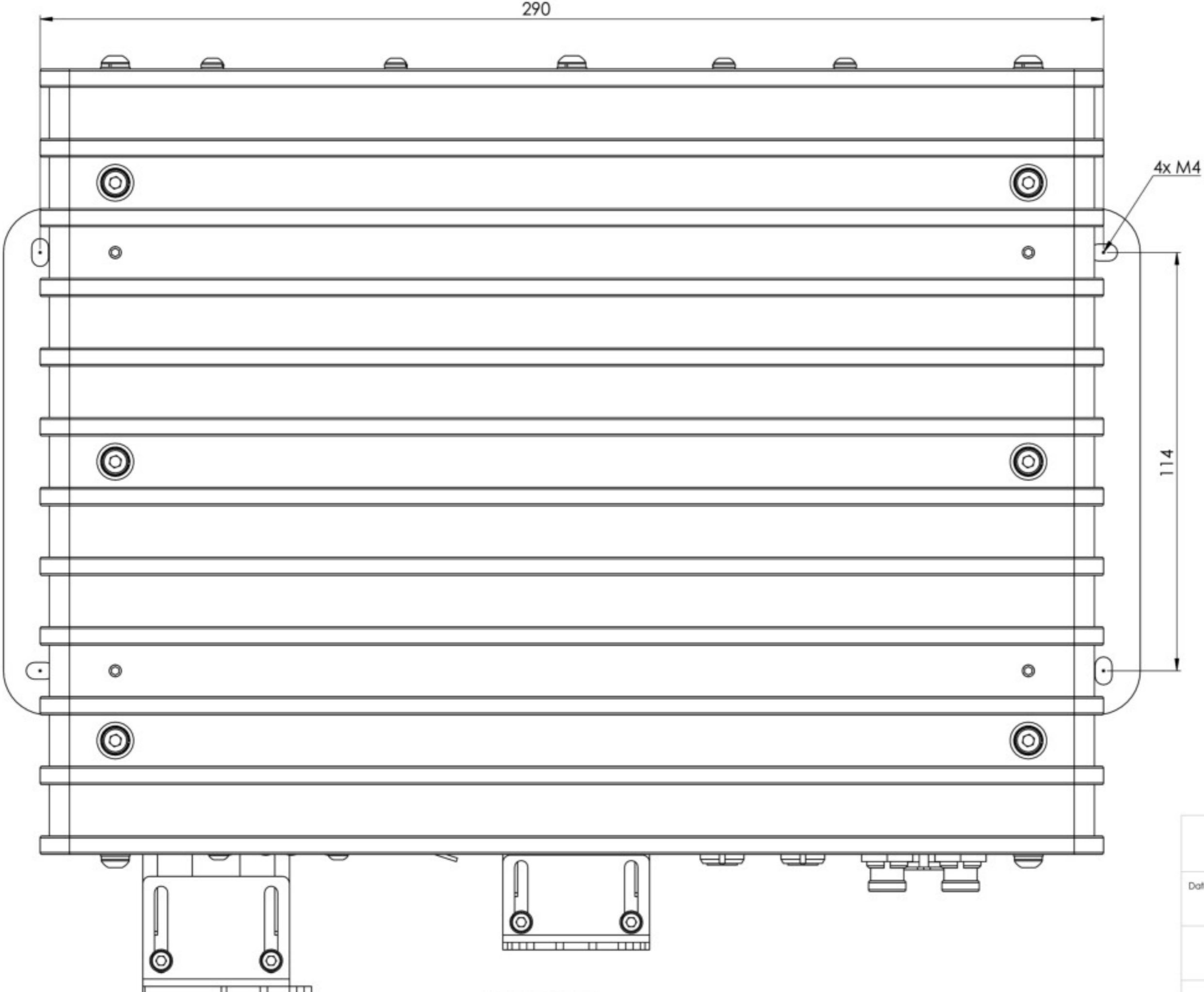
DRILL LAYOUT
