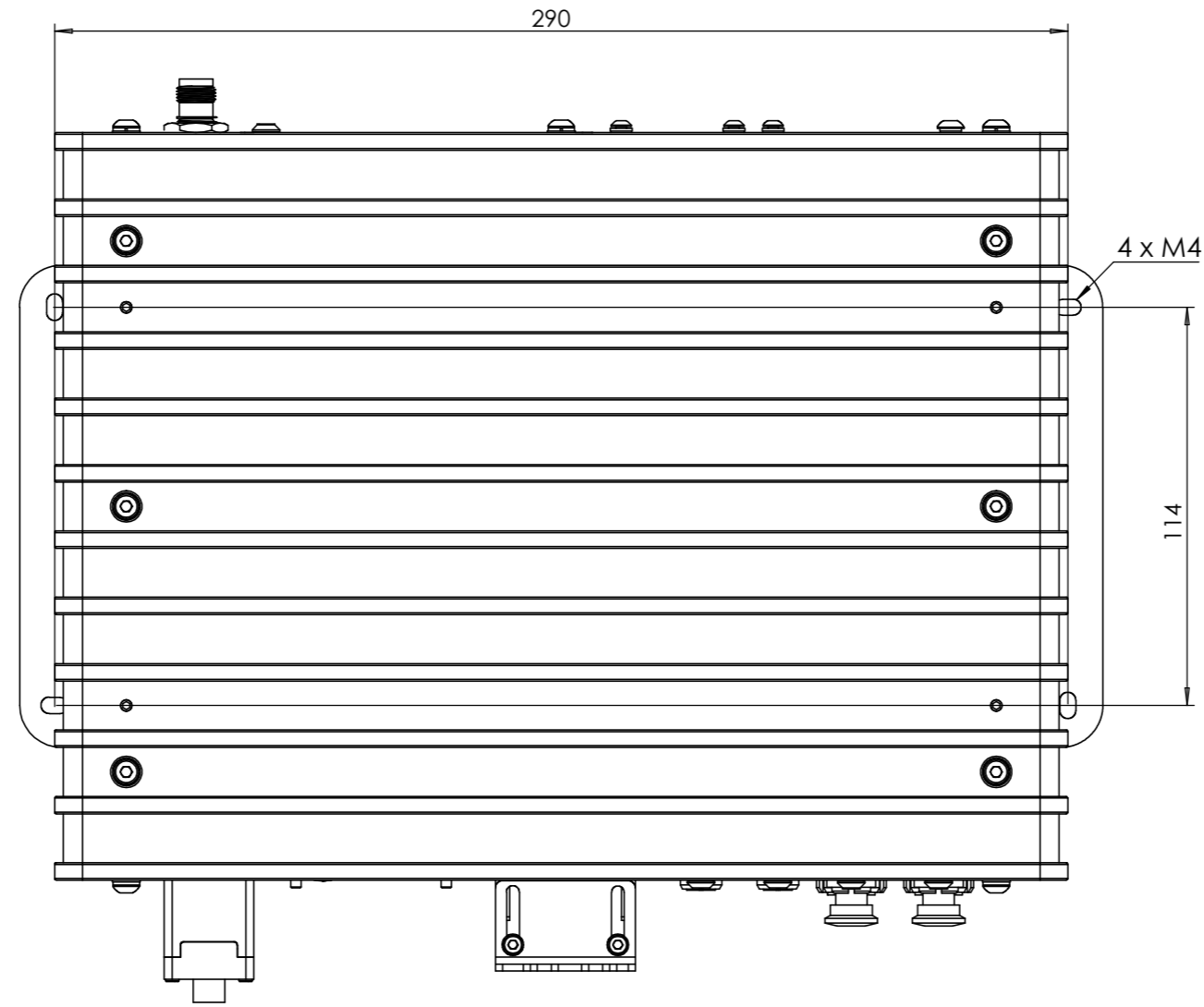
DRILL LAYOUT
